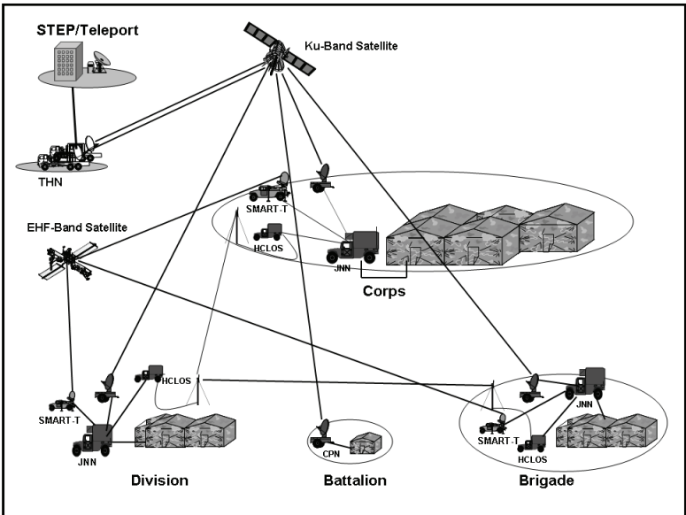
Figure 5-1. WIN-T Increment 1 architecture
